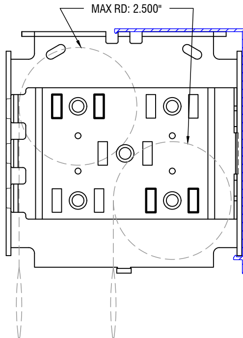
CLUTCH PROFILE
