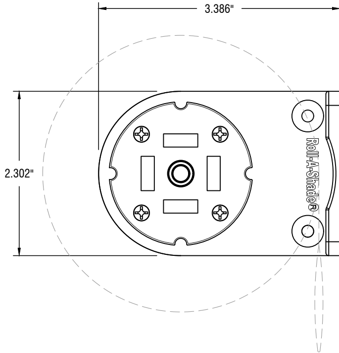
IDLER PROFILE
